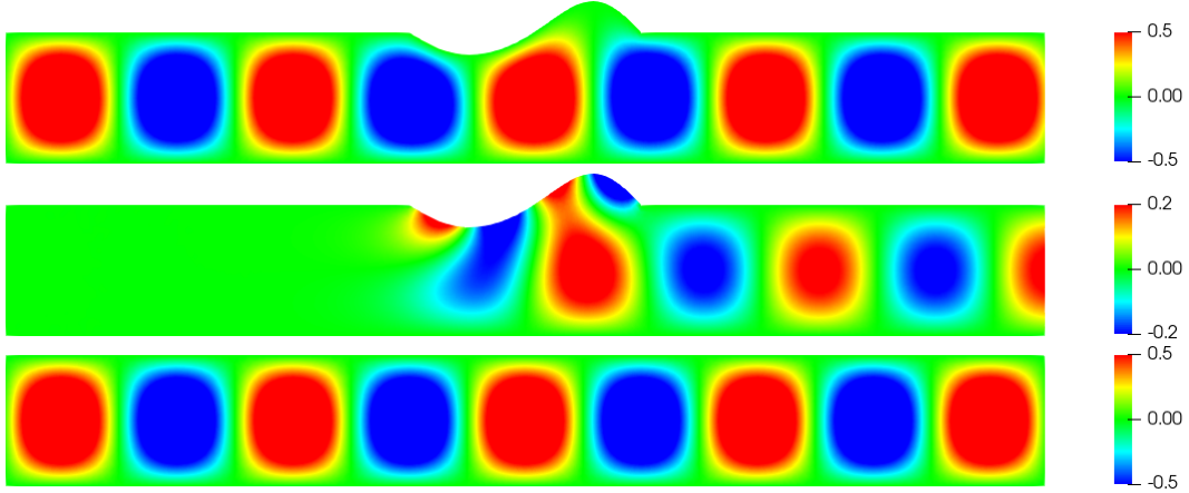
Figure II.2: Example of non reflecting obstacle for the problem (I.67) with Dirichlet BCs. Top: \Re u . Middle: \Re u_s with u_s := u - w_+ . Bottom: \Re w_+ in the reference strip. Here k = 1.5\pi .
