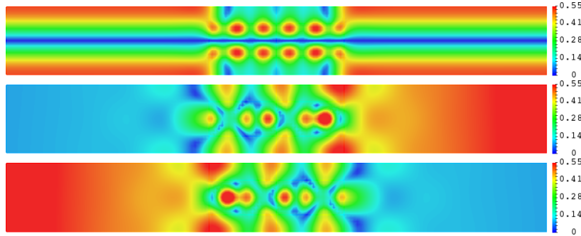
Figure IV.9: Modulus of eigenfunctions of B_\theta associated to the eigenvalues k \approx 5.31 (top), k \approx 5.29 - 0.13i (middle) and k \approx 5.29 + 0.13i (bottom) obtained in Figure IV.6. The symmetry x \rightarrow -x for real k (due to \mathcal{PT} -symmetry) disappears for complex k .
