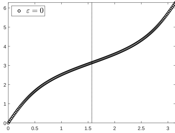
Figure III.3: Map k \mapsto \theta(k) . The vertical black dotted line indicates the value k = \pi/2 .
