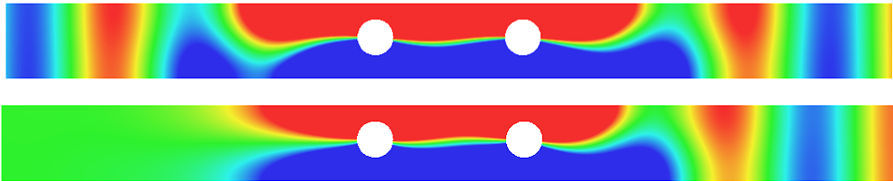
Figure III.12: \Re u^{\varepsilon} (top) and \Re(u^{\varepsilon} - w_{+}) in a setting where R_{\pm}^{\varepsilon} = 0 ( \varepsilon = 0.05 and k = \sqrt{\lambda} = 2.751 ).
