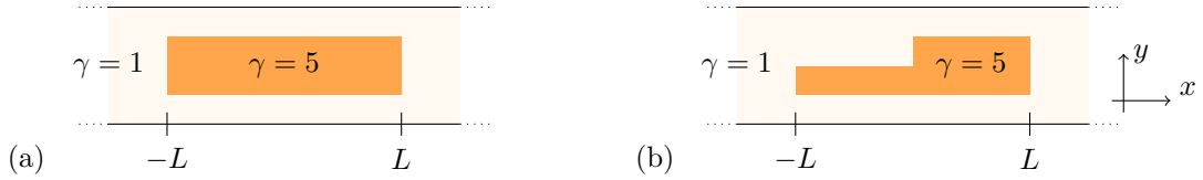
Figure IV.3: Symmetric (a) and non-symmetric (b) obstacles considered in the numerics below.
