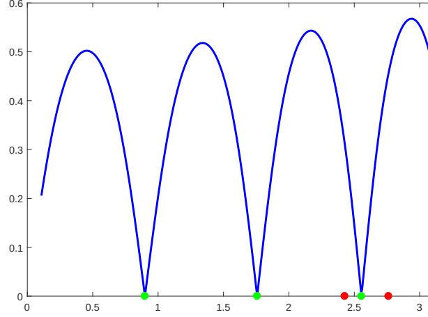
Figure IV.8: Curve k \mapsto |R(k)| (modulus of the reflection coefficient) for k \in (0.1; 3.1) . The green and red dots represent respectively the reflectionless modes and the trapped modes computed in Figure IV.6. We indeed observe that R(k) is null for reflectionless k .
