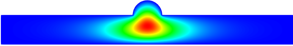
Figure I.3: Example of trapped mode for Problem (I.3). The above function belongs to the kernel of A(k) , i.e. it is an element of H_0^1(\Omega) \setminus \{0\} which satisfies \Delta u + k^2 u = 0 in \Omega , for a certain k > 0 .
