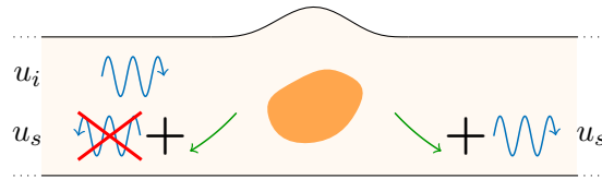
Figure IV.2: Schematic picture of a reflectionless mode. The propagating wave (blue) is not reflected. The backscattered field is purely evanescent (green).
