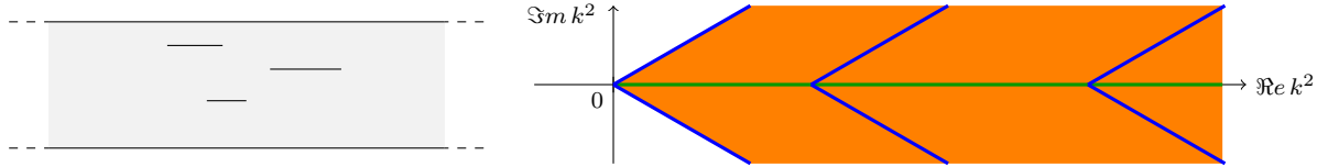
Figure IV.4: Left: waveguide with horizontal cracks. Right: the spectrum of the corresponding B_\theta fills the whole sector delimited by \sigma_{\text{ess}}(B_\theta) . Here the blue lines represent \sigma_{\text{ess}}(B_\theta) .
