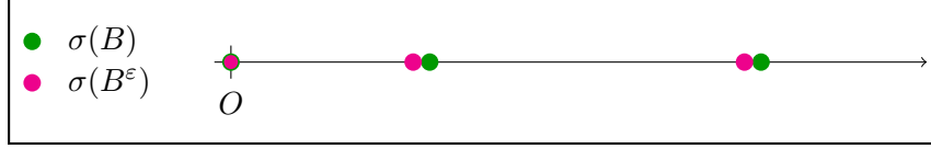
Figure III.9: Spectra of B and B^\varepsilon in the complex plane.
