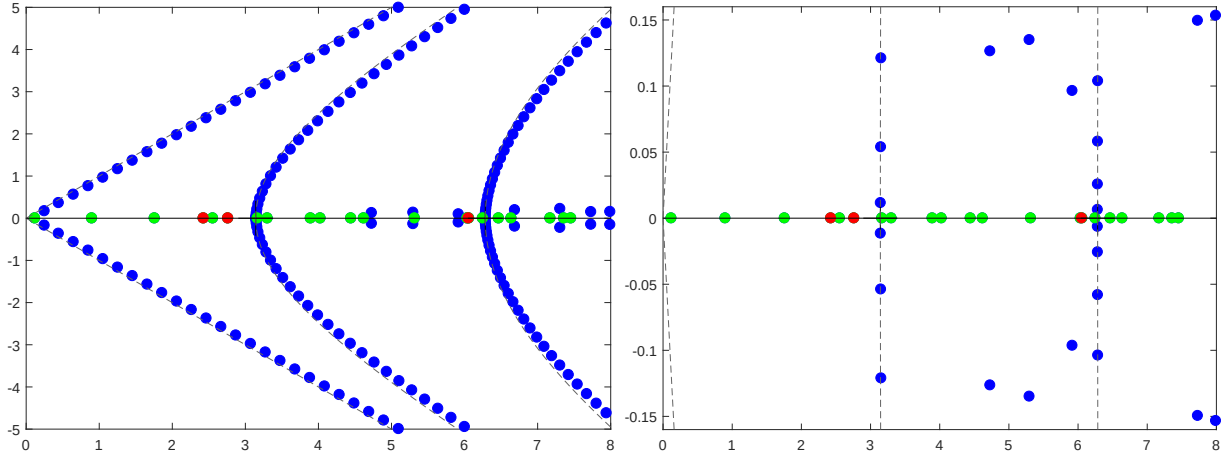
Figure IV.6: Reflectionless eigenvalues in the complex k plane corresponding to the spectrum of B_\theta for a symmetric obstacle (Figure IV.3 (a)). The trapped modes in red are the same as in Figure IV.5. The reflectionless modes are in green and the dashed lines represent the essential spectrum of B_\theta (see (IV.19)). The picture on the right is a zoom-in of that on the left.
