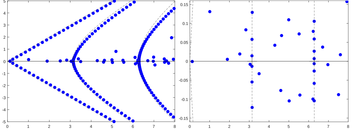
Figure IV.10: Spectrum of B_\theta in the complex k plane for a non symmetric obstacle (Figure IV.3 (b)). The dashed lines represent the essential spectrum of B_\theta (see (IV.19)). The spectrum is not stable by conjugation. The picture on the right is a zoom-in of that on the left.
