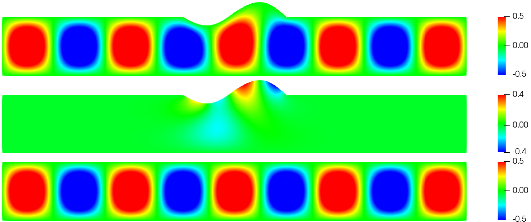
Figure II.3: Example of perfectly invisible obstacle for the problem (I.67) with Dirichlet BCs. Top: \Re u . Middle: \Re u_s . Bottom: \Re w_+ in the reference strip. Here k = 1.5\pi .
