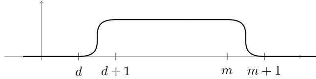
Figure I.4: Graph of the cut-off function \psi_m .
