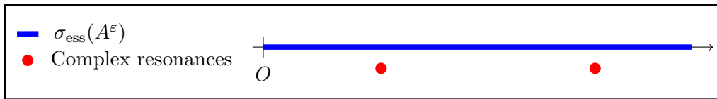
Figure III.8: Spectrum of A^\varepsilon in the complex plane.
