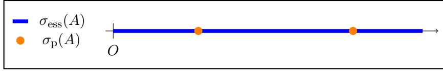
Figure III.4: Spectrum of A in the complex plane.
