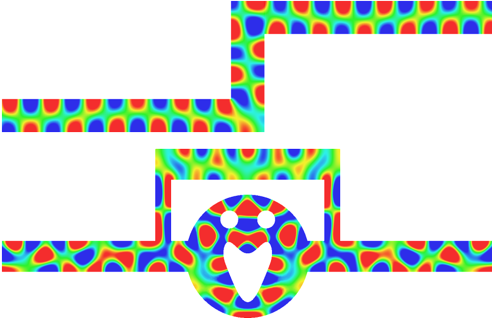
Figure IV.12: Examples of reflectionless modes in waveguides with sound hard walls (Neumann).
