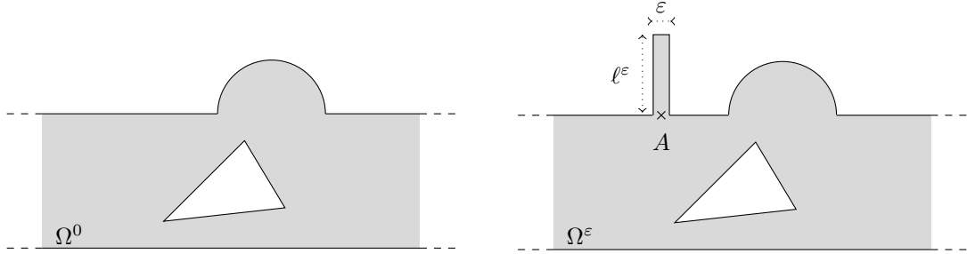
Figure III.15: Left: initial setting. Right: geometry with one thin outer resonator.
