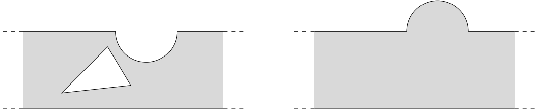
Figure I.2: Left: example of domain where A(k) is an isomorphism for all k \in (0; \pi) . Right: example of domain where one can show that A(k) is not an isomorphism for all k \in (0; \pi) .
