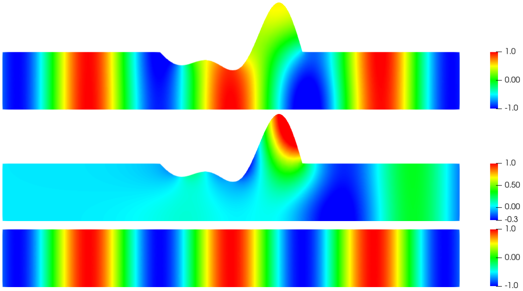
Figure II.4: Example of non reflecting geometry for Problem (I.77) with Neumann BCs. Top: \Re u . Middle: \Re u_s . Bottom: \Re w_+ in the reference strip. Here k = 0.8\pi .
