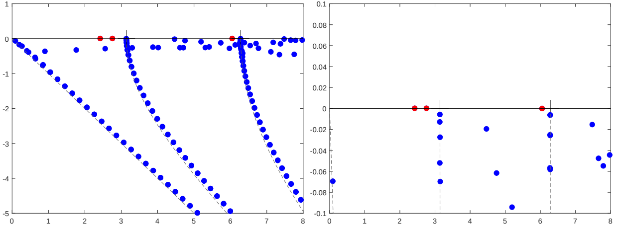
Figure IV.5: Classical complex resonances in the complex k plane corresponding to the spectrum of A_\theta for a symmetric obstacle (Figure IV.3 (a)). The trapped modes are in red, the dashed lines represent the essential spectrum of A_\theta (see (IV.15)). The picture on the right is a zoom-in of that on the left.
