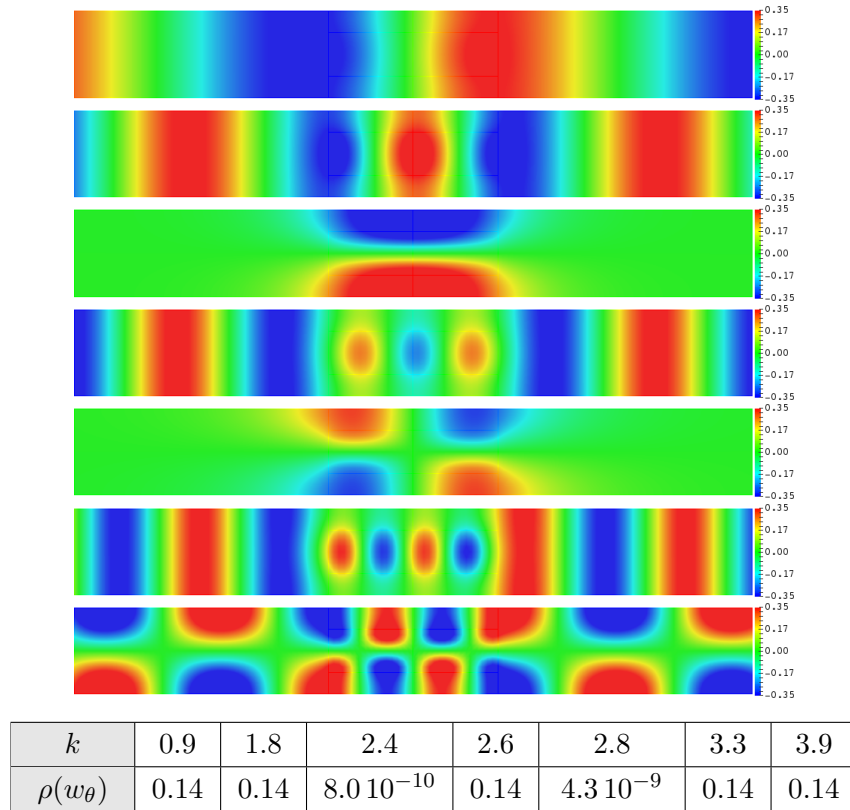
Figure IV.7: Top: real part of eigenmodes associated with real eigenvalues of B_\theta from Figure IV.6. Bottom: value of k and of the indicator function \rho for each of these 7 eigenmodes. The 3rd and the 5th eigenmodes are trapped modes, the five others are reflectionless modes.
