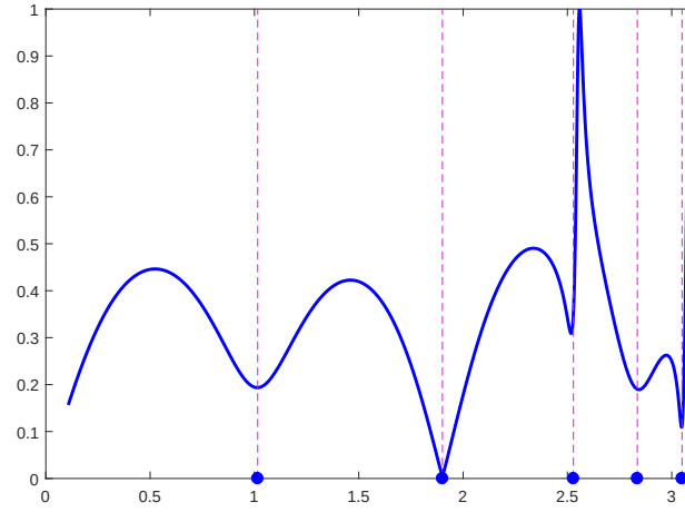
Figure IV.11: Curve k \mapsto |R(k)| (modulus of the reflection coefficient) for k \in (0.1; 3.1) and a non symmetric obstacle. The blue dots and the vertical dashed lines correspond to the real parts of the eigenvalues of B_\theta located close to the real axis computed in Figure IV.10. We observe that |R(k)| is minimal for these particular k .
