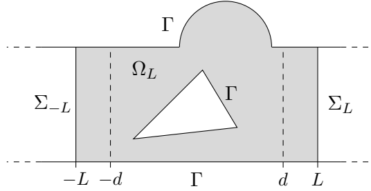
Figure I.5: Domain \Omega_L .
